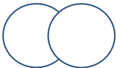
Chlorine
